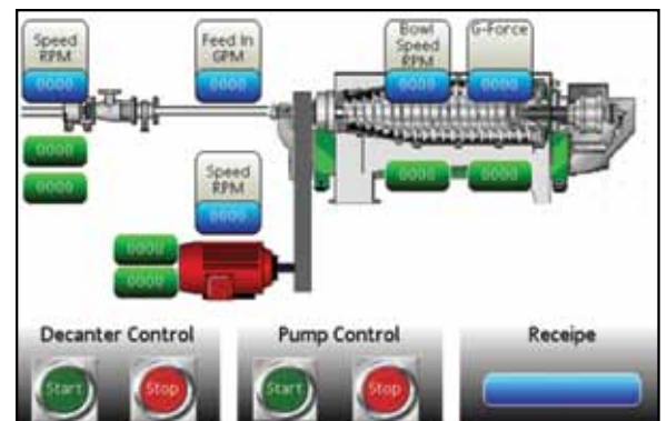
Figure 14 – KEMTRON’s DFD Systems Incorporate Dual Polymer Feed Tanks and Dual Mix Tanks
