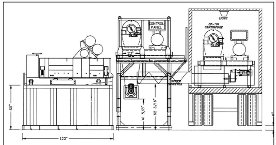
Figure 3 – Cross-Section of KEMTRON's DFD System Using a Trailer-Mounted Dewatering Package.
