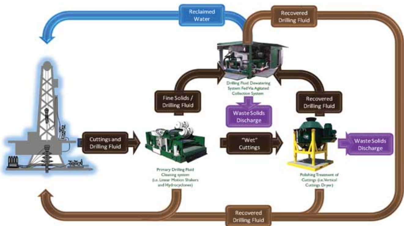
Figure 6 – KEMTRON’s DFD System Combined with a Primary and Secondary Solids Control System
