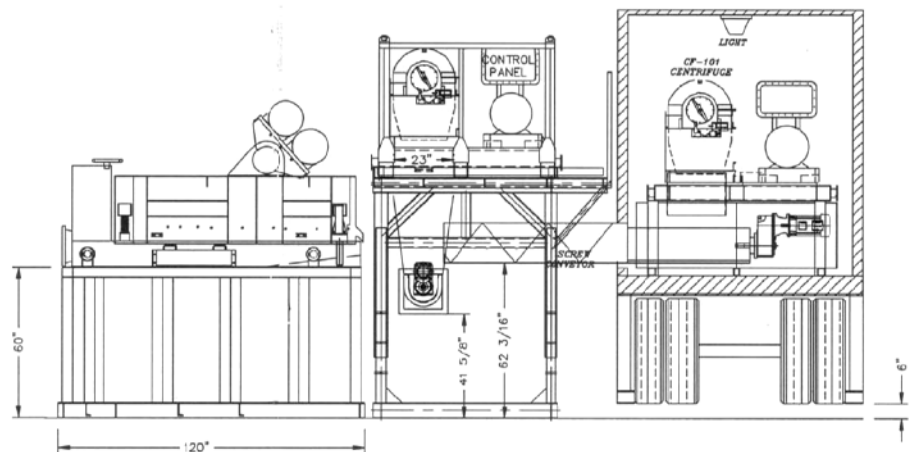
Figure 3 – Cross-Section of KEM-TRON’s DFD System Using a Trailer-Mounted Dewatering Package.
