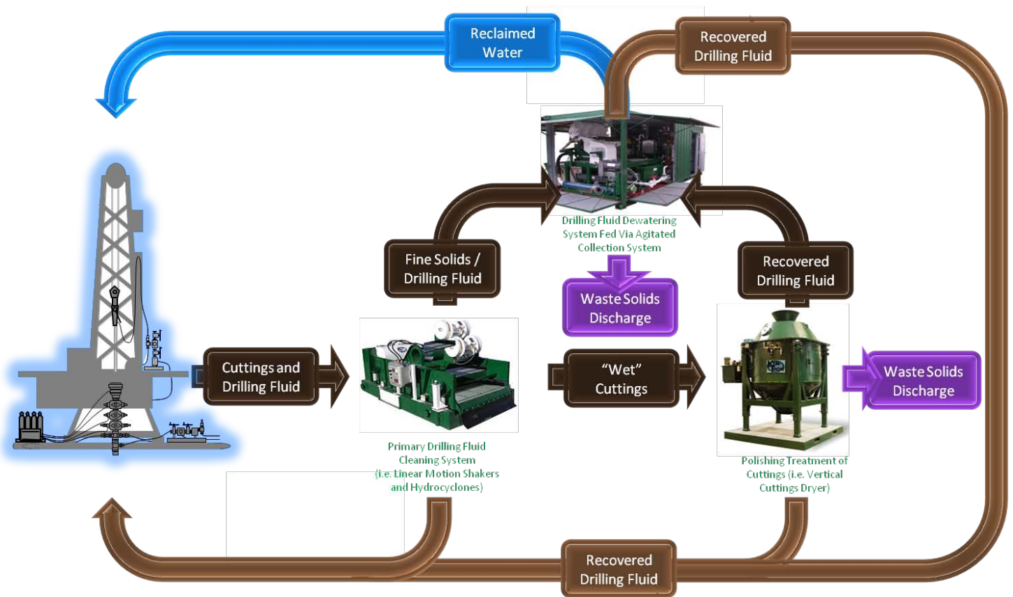
Figure 6 – KEM-TRON’s DFD System Combined with a Primary and Secondary Solids Control System
